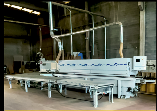
Brandt / 2012 Ligmatech KDF 670 Profiline single sided edgebander
